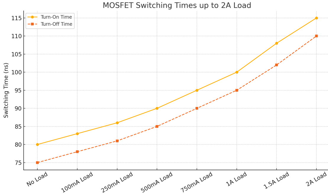
Figure x: Figure X: MOSFET Switching Times as a Function of Load Current
