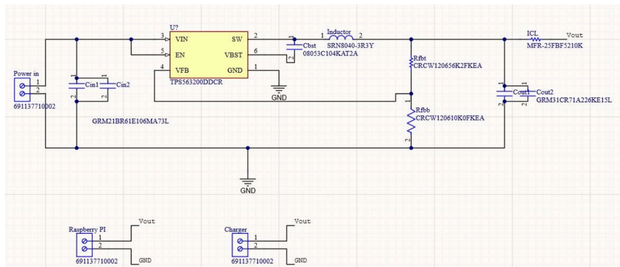
Figure x: Buck Converter Altium Circuit Schematic
