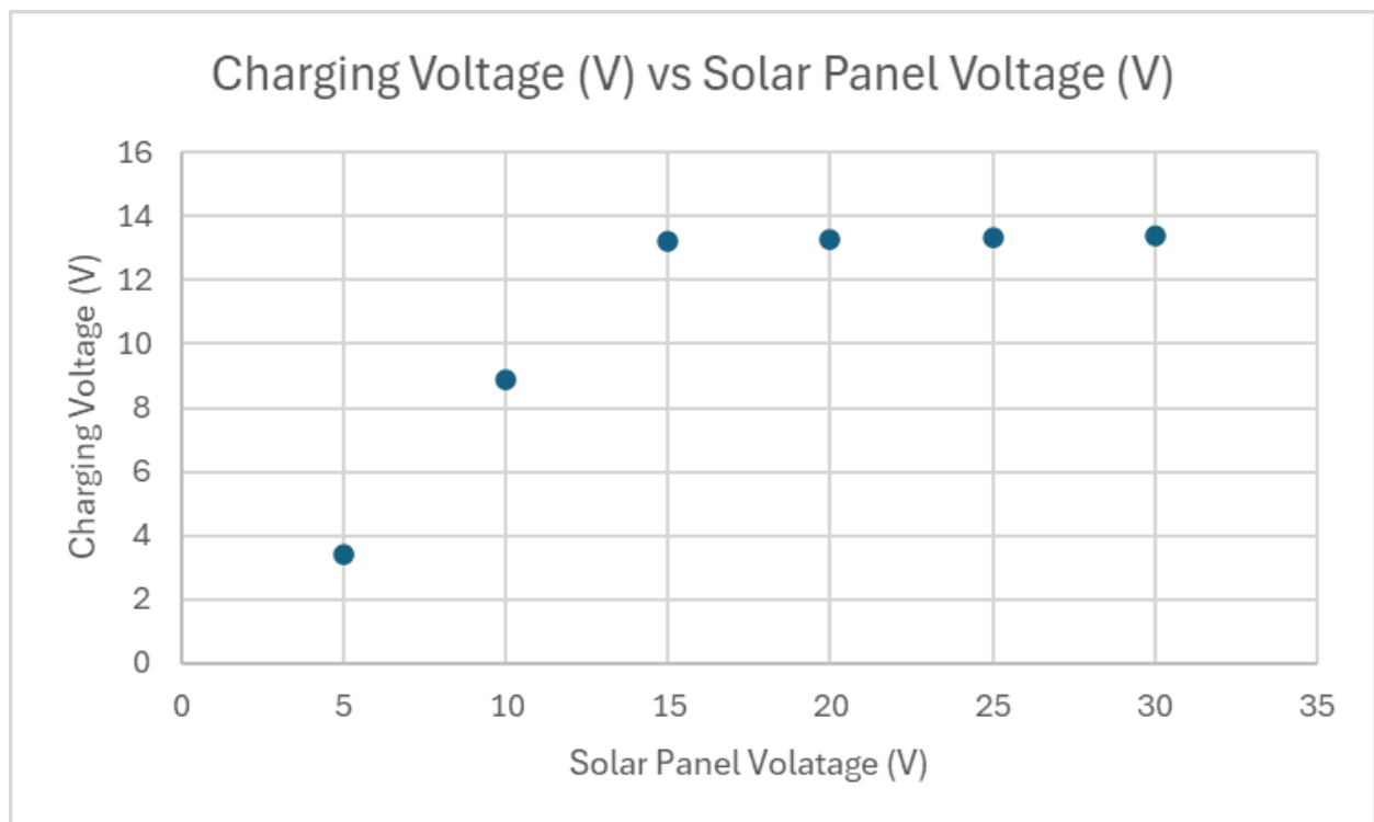
Figure 7: Simulated Solar Inputs vs Charging Voltage
