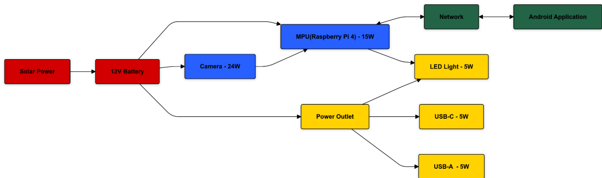
Figure 2: SolarEye Security System Block Diagram
