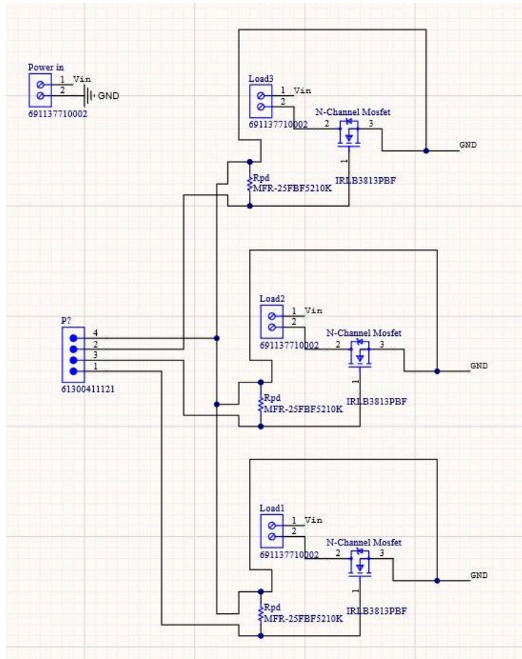
Figure x: Relay Control Module Altium Circuit Schematic
