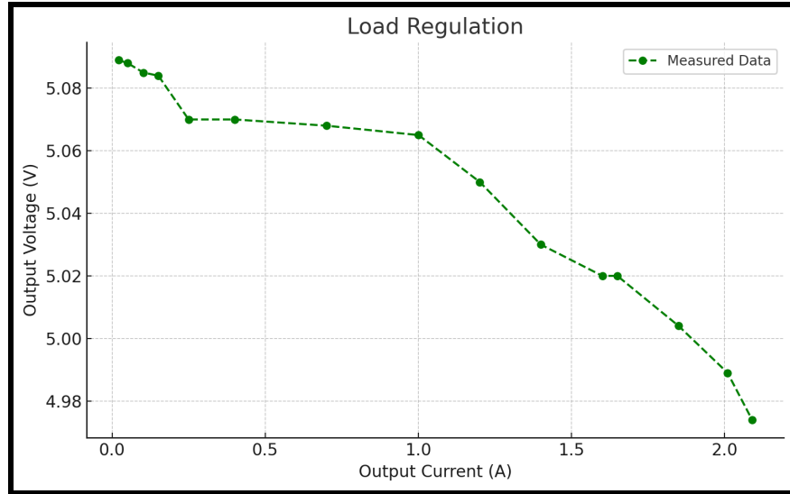
Figure x: Buck Load Regulation
