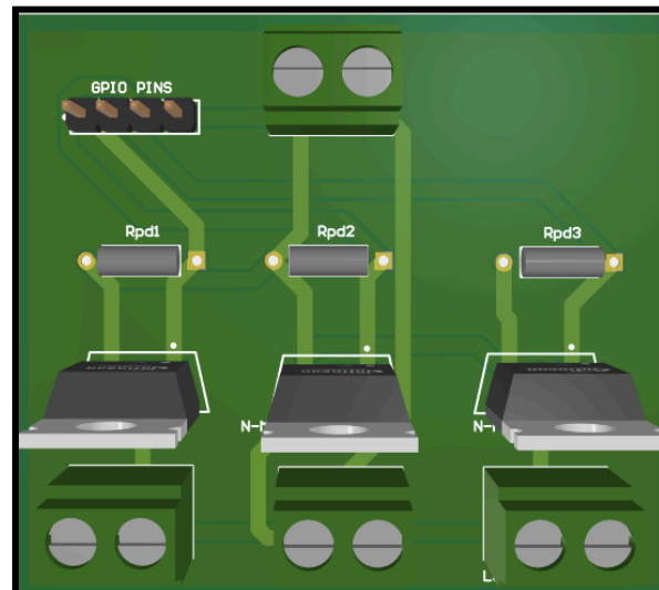
Figure x: Relay Control Module PCB
