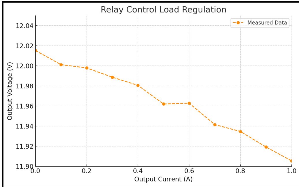
Figure x: Relay Control Module Load regulation
