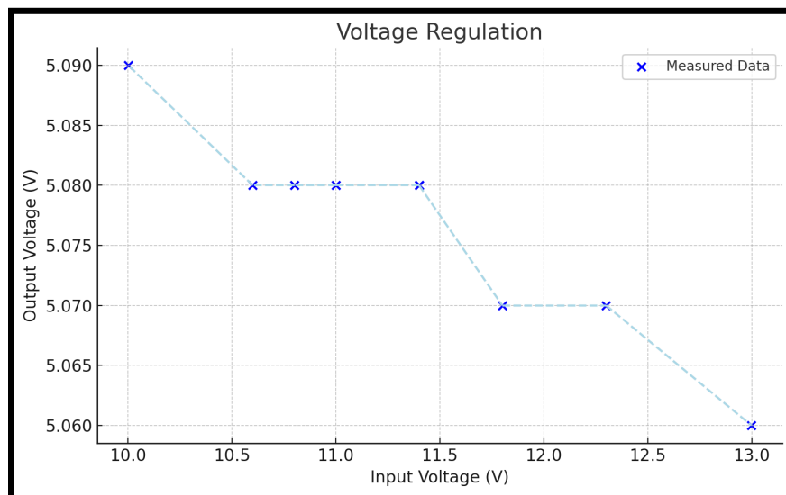
Figure x: Buck Voltage regulation
