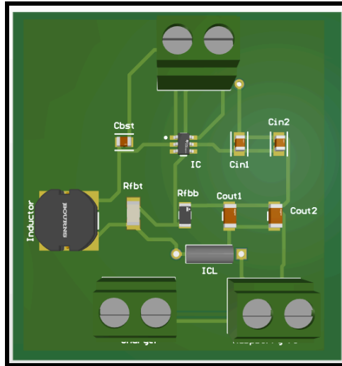
Figure x: Buck Converter
